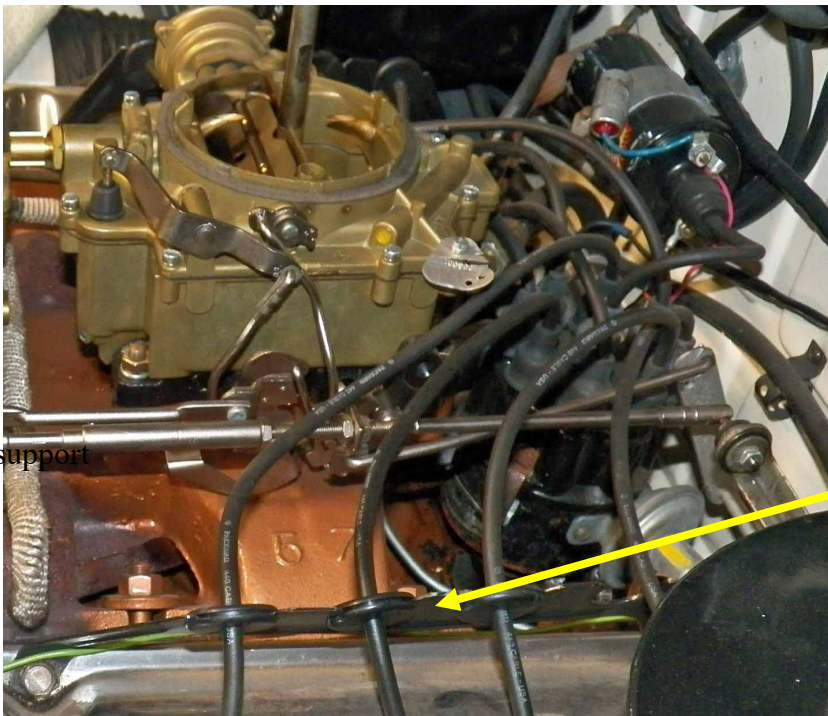
1955 Packard Clipper engine showing location of ignition wire support bracket on LEFT side of engine. The right side also has two. The senior Packard engines have same arrangement. The two rearmost wires on each side are longer than on 1956 Packards and Clippers which use two larger support brackets.
