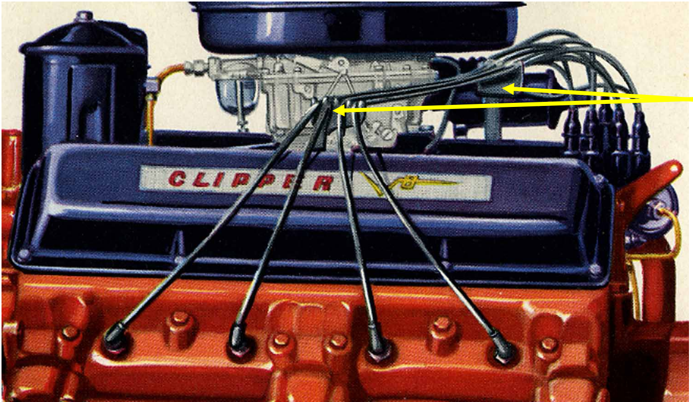
1955 Packard Clipper engine showing location of ignition wire support bracket on LEFT side of engine. The right side also has two. The senior Packard engines have same arrangement. The two rearmost wires on each side are longer than on 1956 Packards and Clippers which use two larger support brackets.
